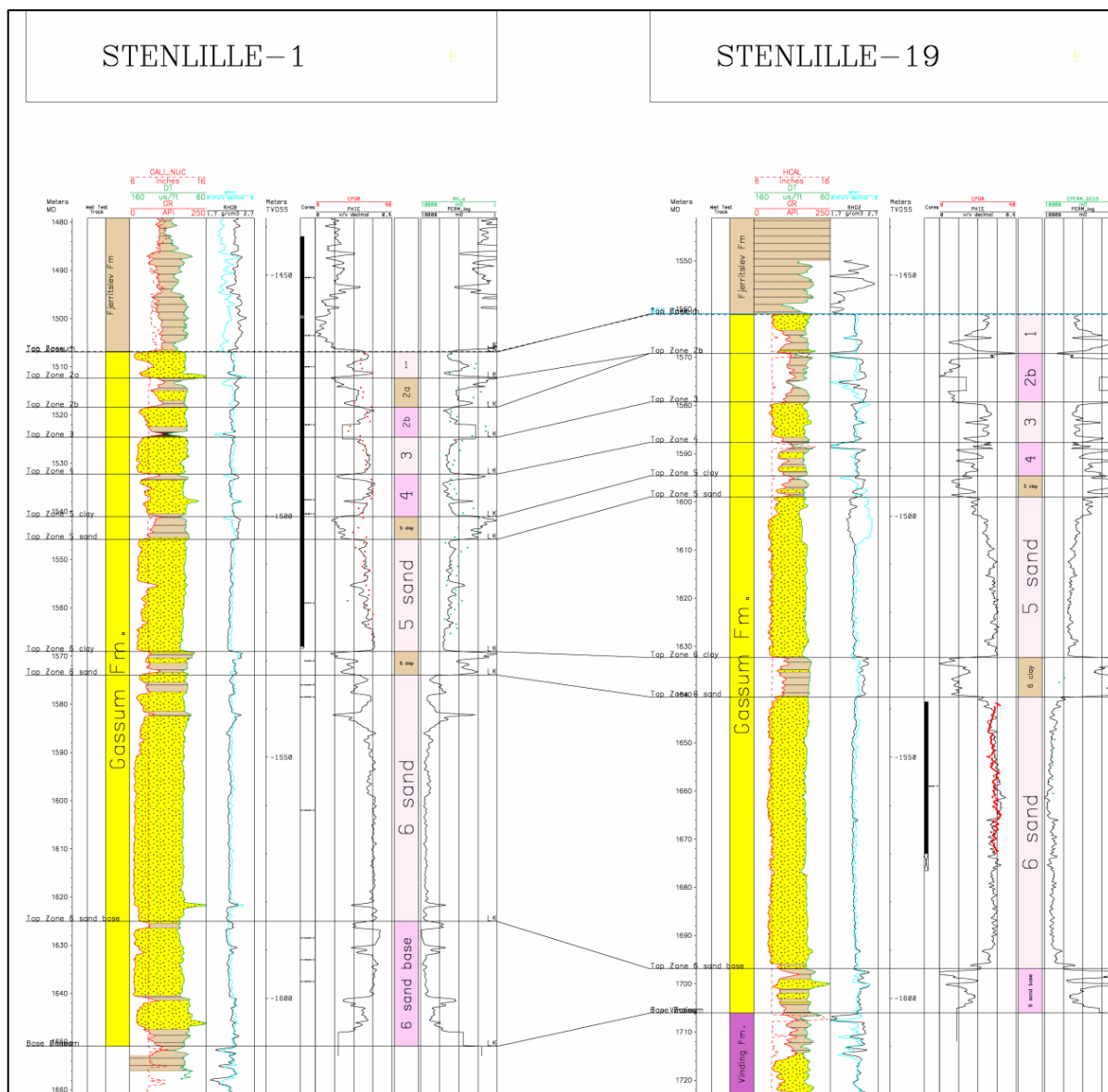
Figure 5. Log correlation and petrophysical evaluation of the Stenlille-1 and Stenlille-19 wells. The plot includes lithological interpretation, lithostratigraphy and subdivision into zones. Interpreted porosity (PHIE) and permeability (PERM_log) are illustrated by curves. Cored intervals indicated by black bars. Core porosity data (red dots, CPOR), and core permeability data (green dots, CPERM or gas permeability, right track) are also shown. Porosity scale: 0–40%, permeability scale: 10000–1 mD. The raw logs plotted are GR: Gamma-ray log, DT: Sonic log, CALI/HCAL: Caliper log, RHOB: Density log, NPHI: Neutron log.
