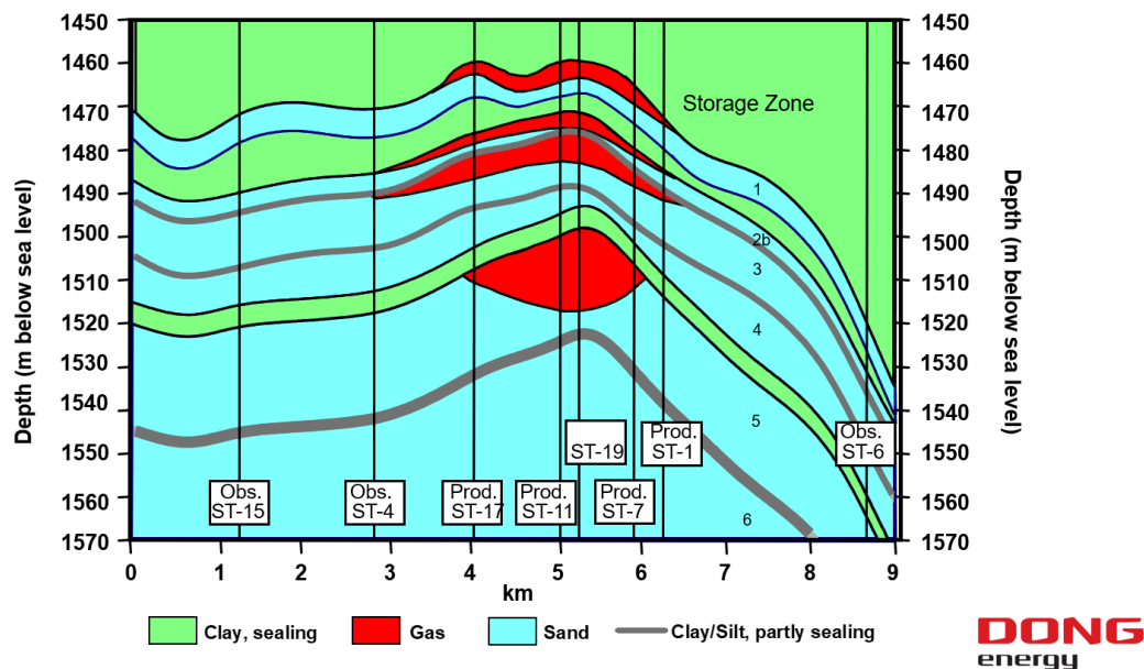
Figure 2: The gas storage facility at Stenlille. Gas is stored in selected zones within the Gassum Formation. The top of the Gassum Formation is found within the depth range 1450–1550 m b. MSL. The distribution of sandstone layers suitable for gas storage, and sealing clay beds, are shown. Figure provided by DONG Energy.
