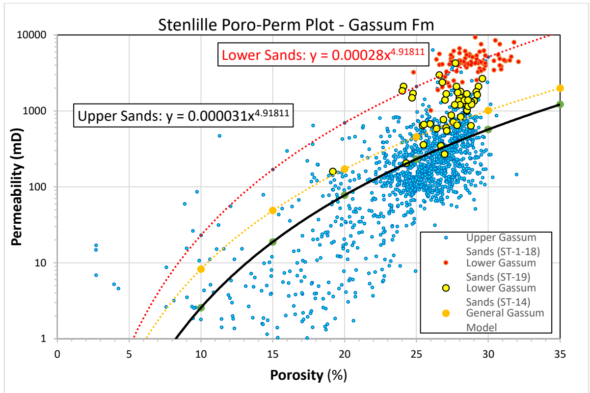
Figure 3: Porosity-permeability relationships for the Gassum Formation sandstones. Based on conventional core analysis data from cored Stenlille wells. The black line represents the upper part of the Gassum Formation, the red line represents the lower part of the Gassum Formation. Permeability values are gas permeabilities measured in a core laboratory (GEUS, COREX etc.). The data points in orange and the orange trend line refer to the General GEUS Poro-Perm Model representing the Gassum Formation outside the Stenlille area (included for comparison).
