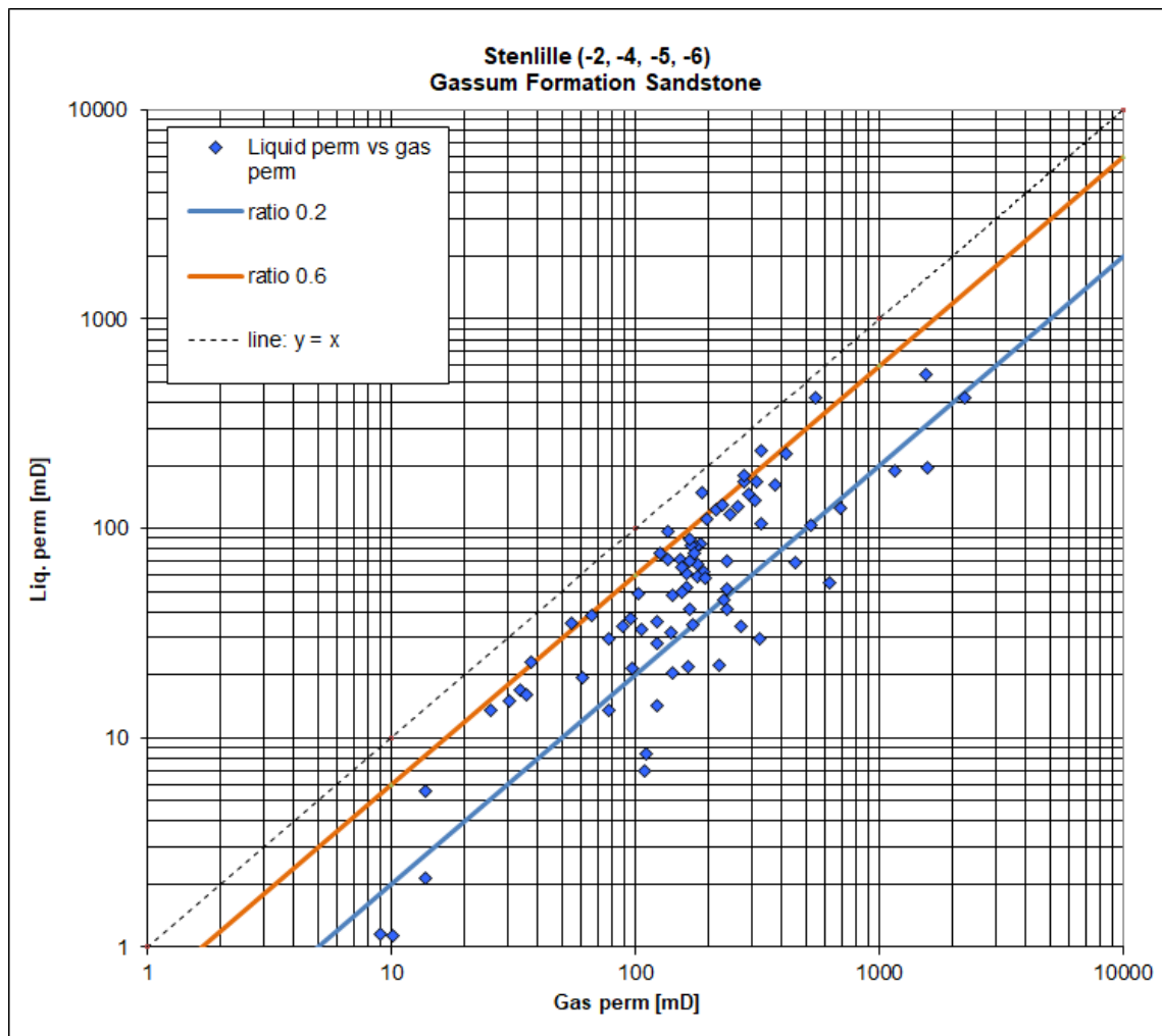
Figure 4: Relationship between gas permeability and liquid permeability. Based on core analysis data from the Stenlille-2, -4, -5 and 6 wells.
