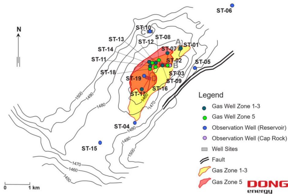
Stenlille Gas Storage - Top Gassum Formation (mbMSL)
